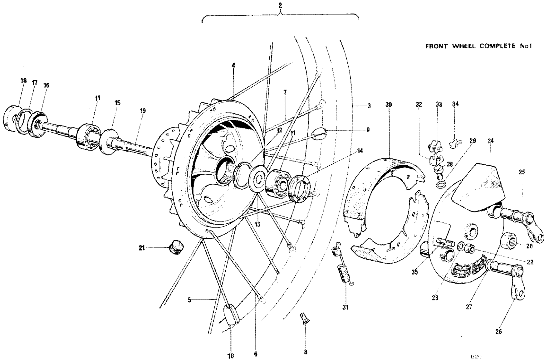
Fig. 22. FRONT WHEEL
