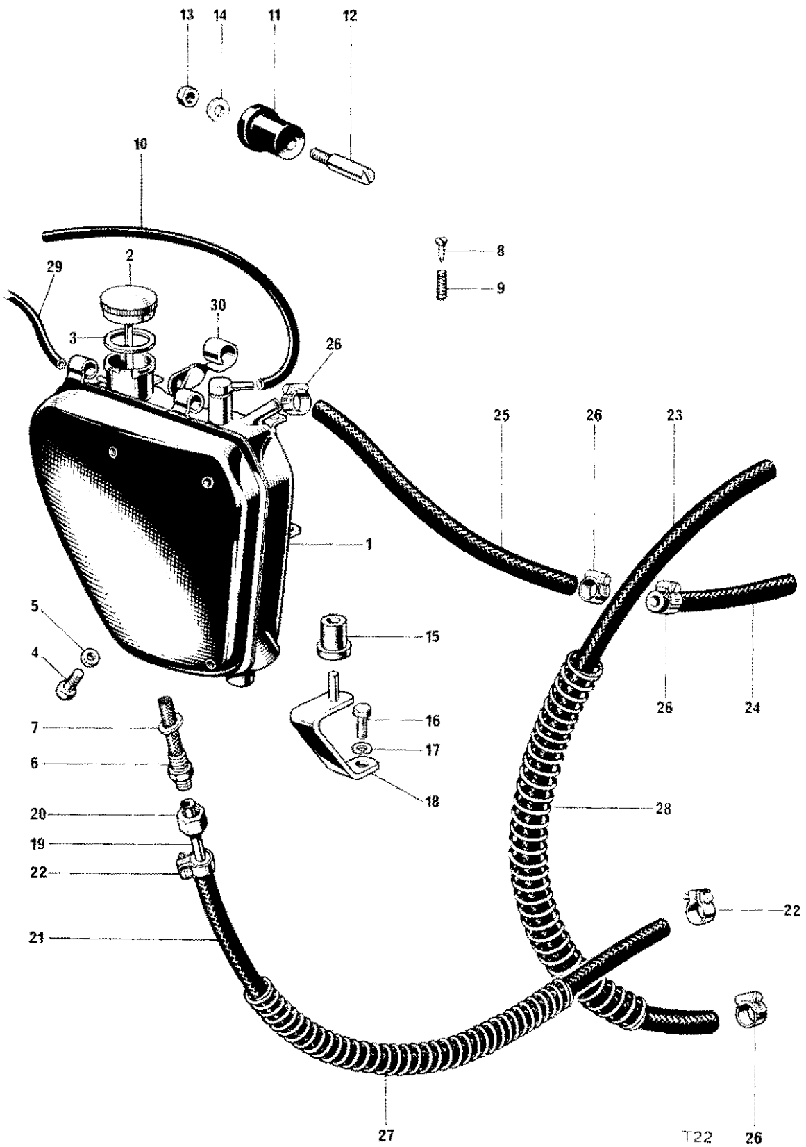
Fig. 26. OIL TANK
