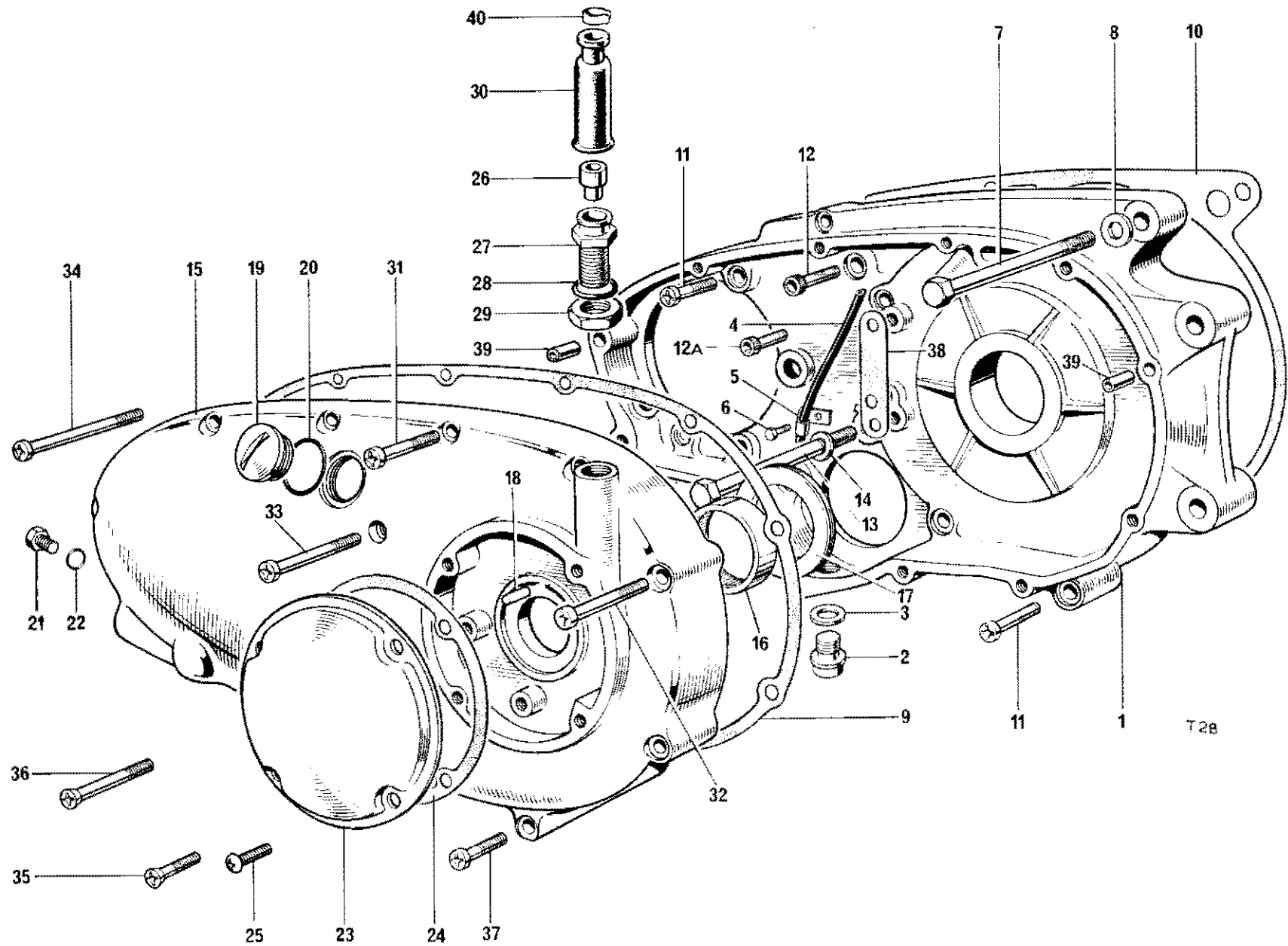
Fig. 14. INNER AND OUTER CHAINCASE
