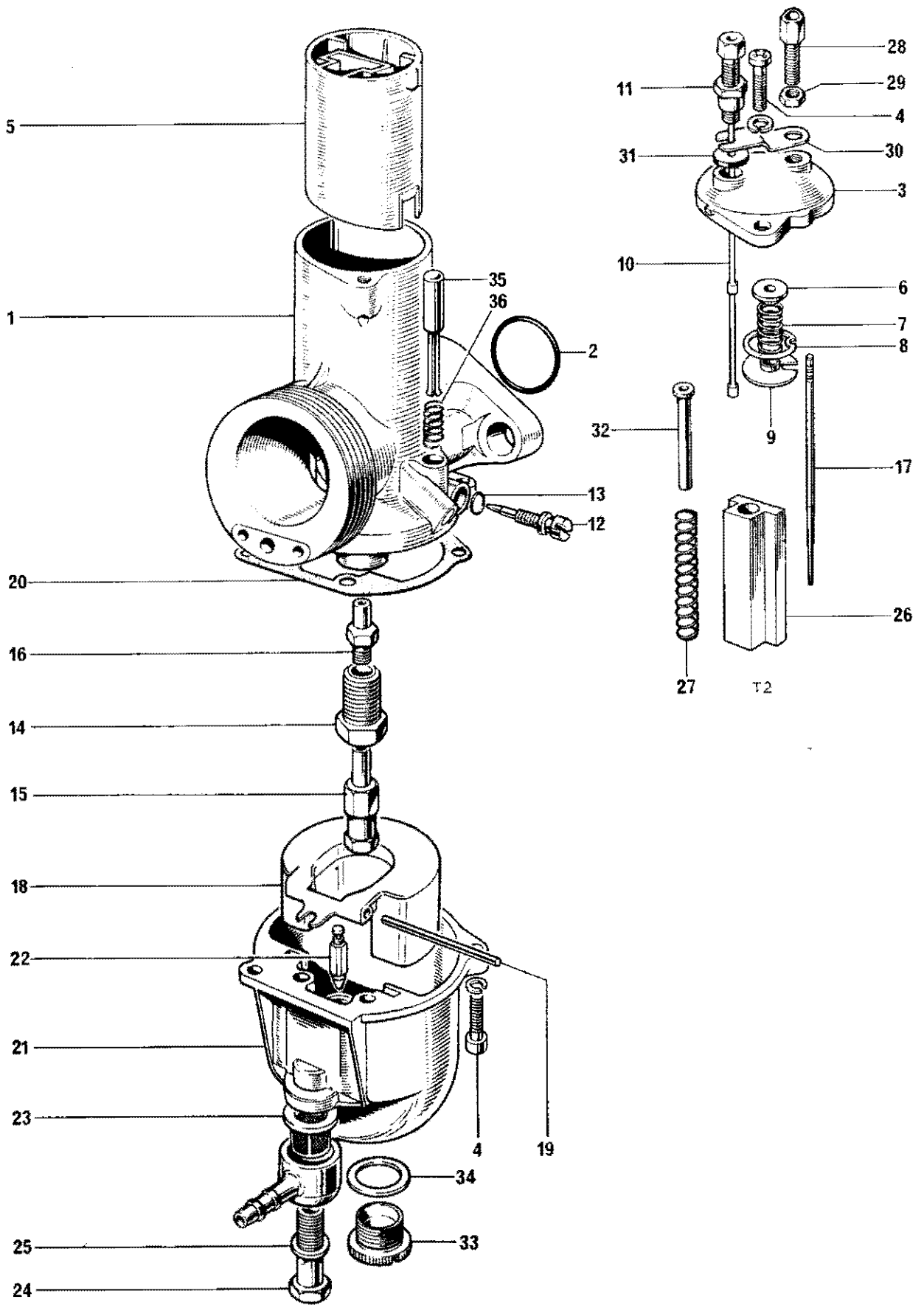
Fig. 5. CARBURETORS
