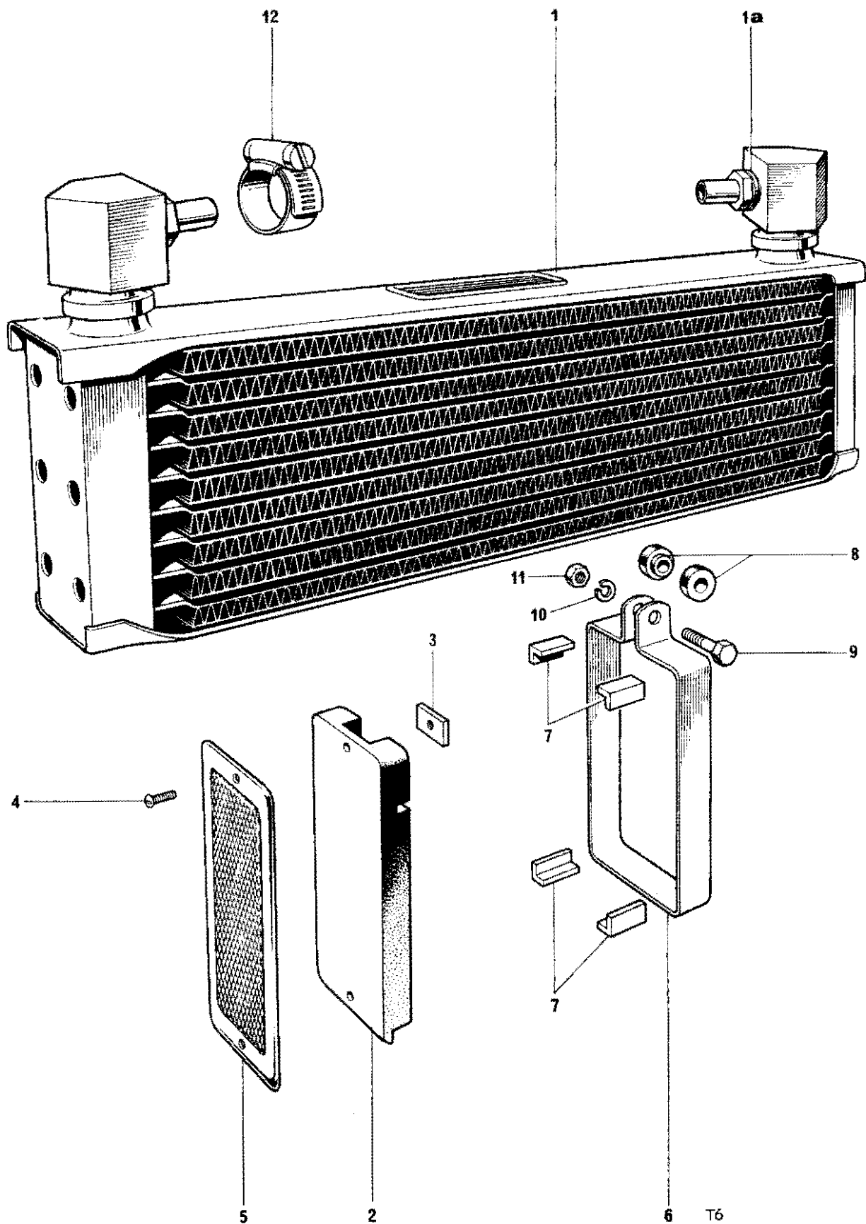
Fig. 24. OIL COOLER
