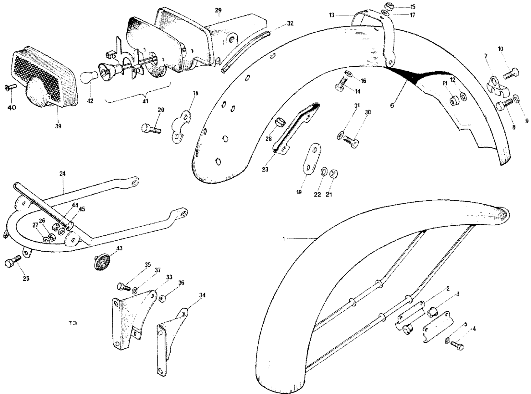
Fig. 29. FENDERS AND TAIL LAMP
