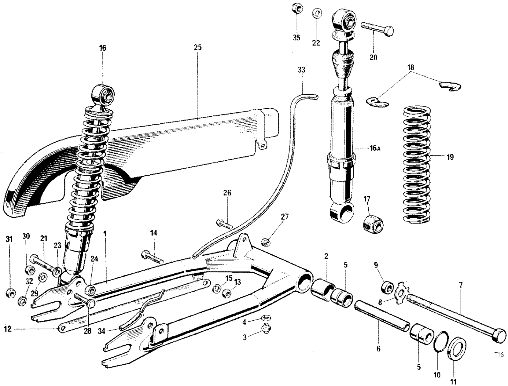
Fig. 17. SWINGING FORK AND SUSPENSION UNITS
