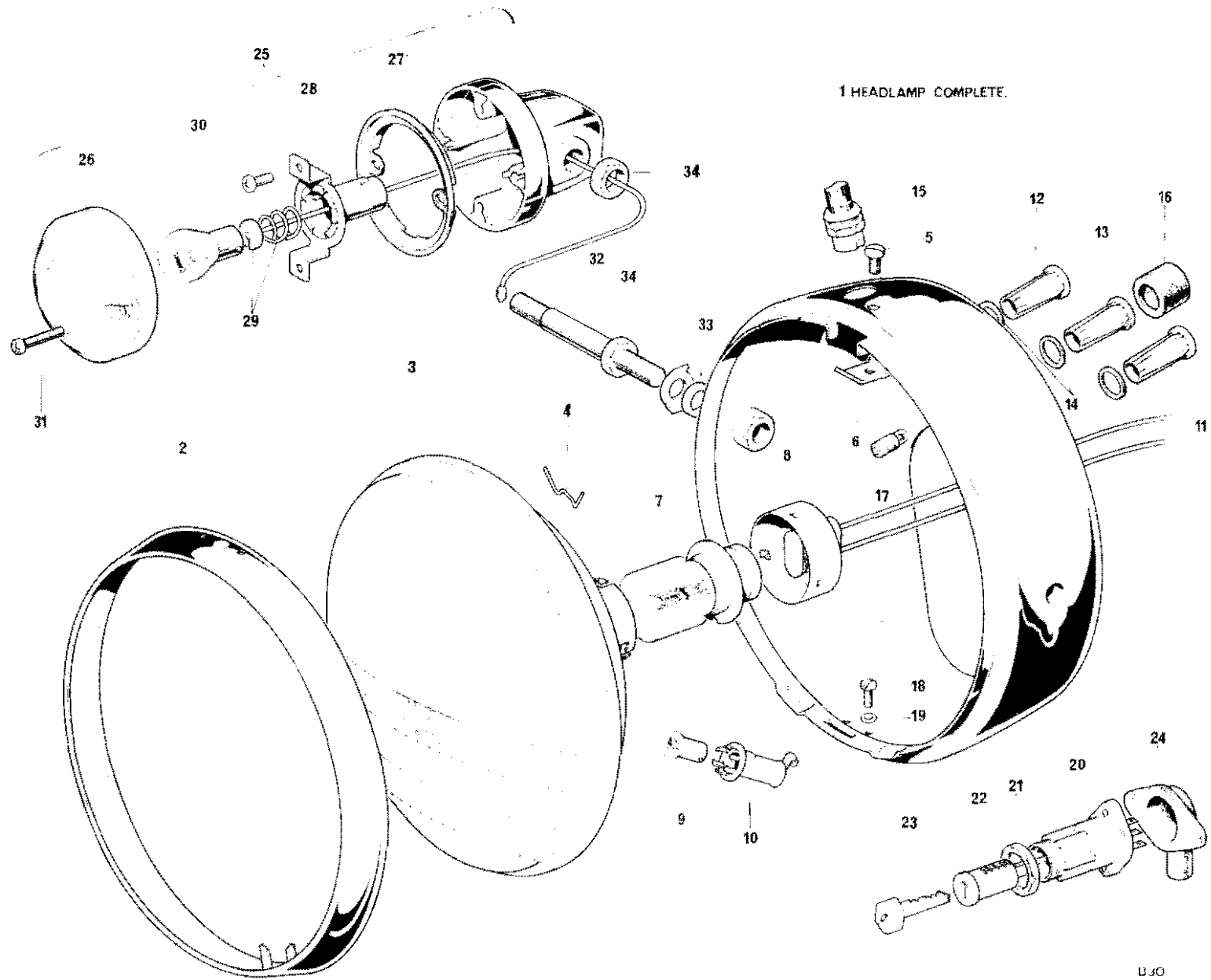
Fig. 32. HEADLAMP AND FLASHER LAMPS
