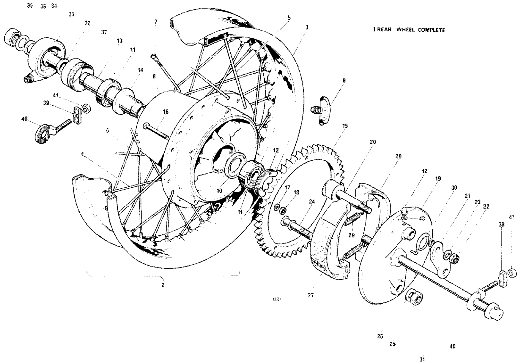
Fig. 23. REAR WHEEL
