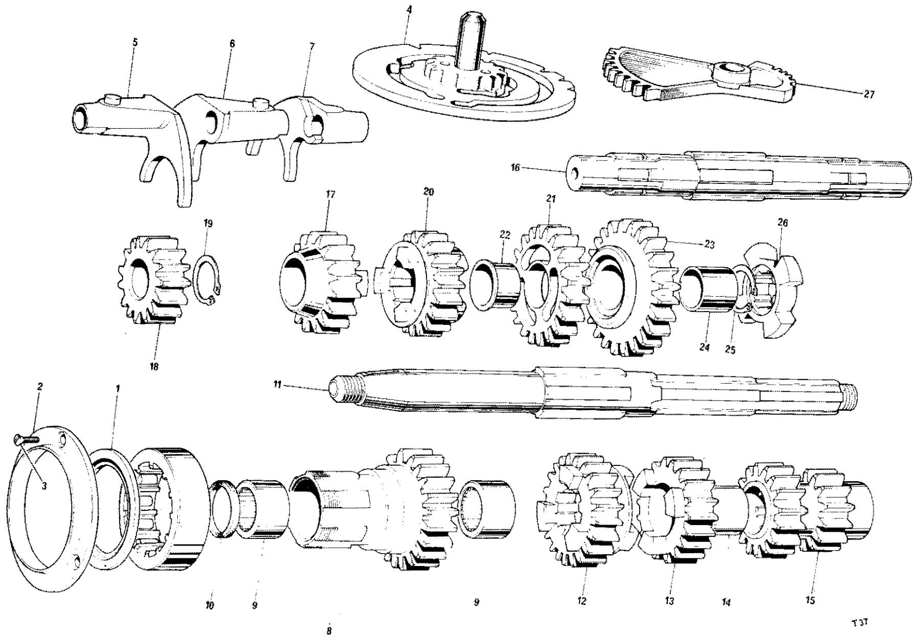
Fig. 12. GEARBOX SHAFTS AND GEARS—T150V (5 SPEED)
