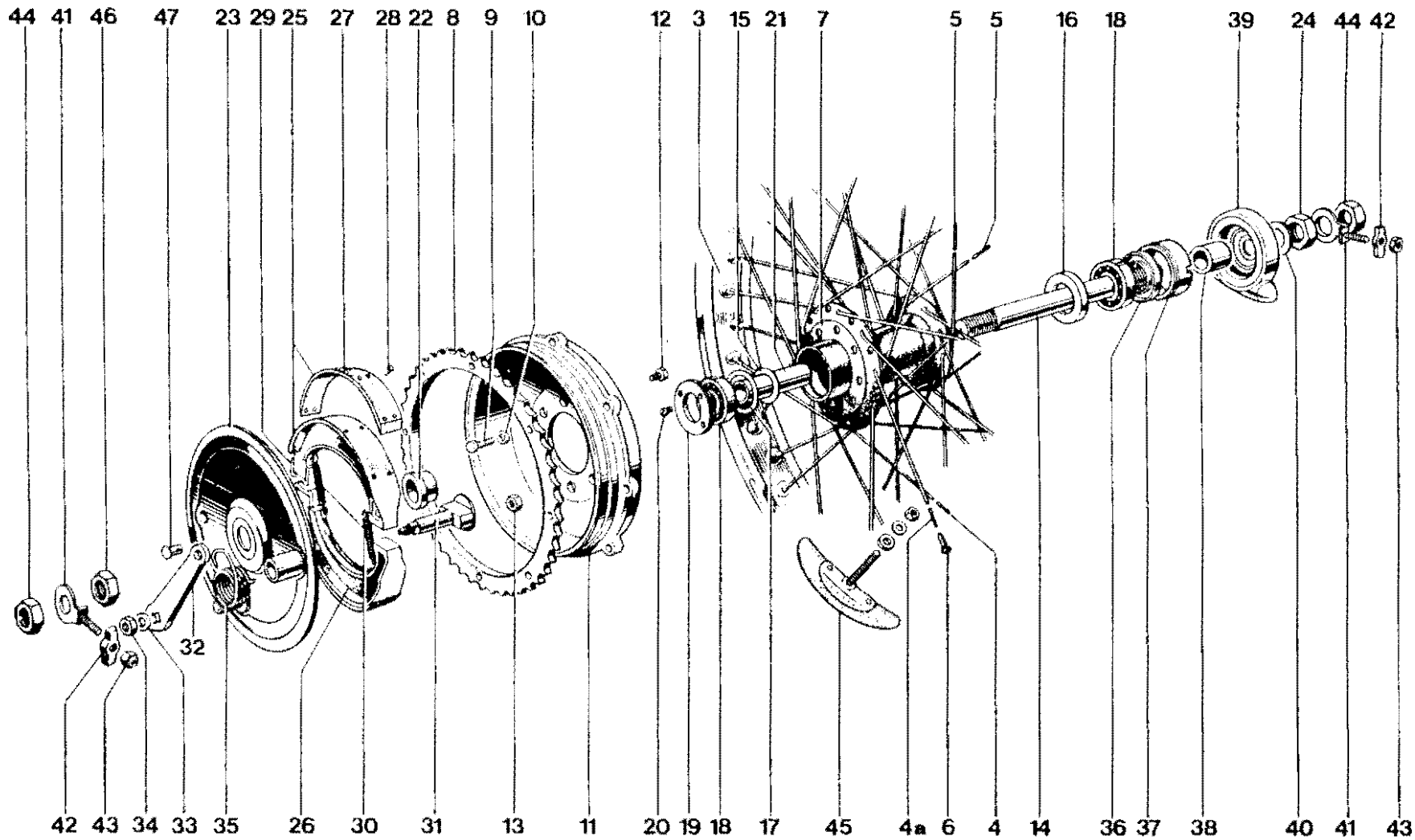
Fig. 20. REAR WHEEL
