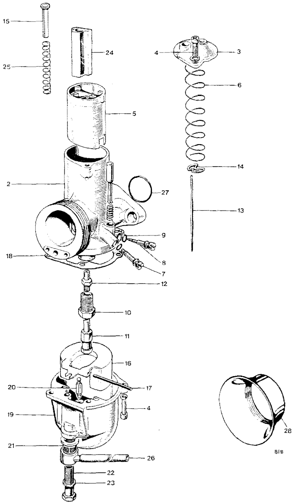
Fig. 29. AMAL CARURETOR, TR6R, TR6C
