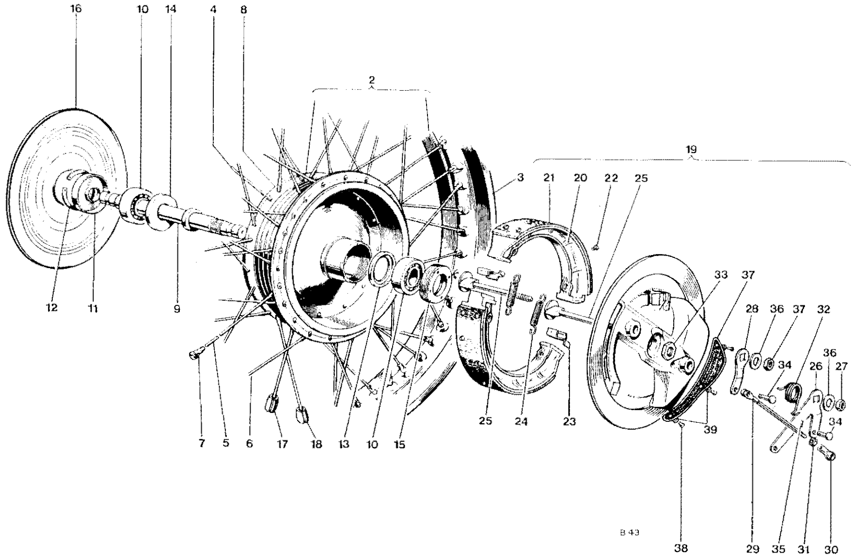
Fig. 19. FRONT WHEEL
